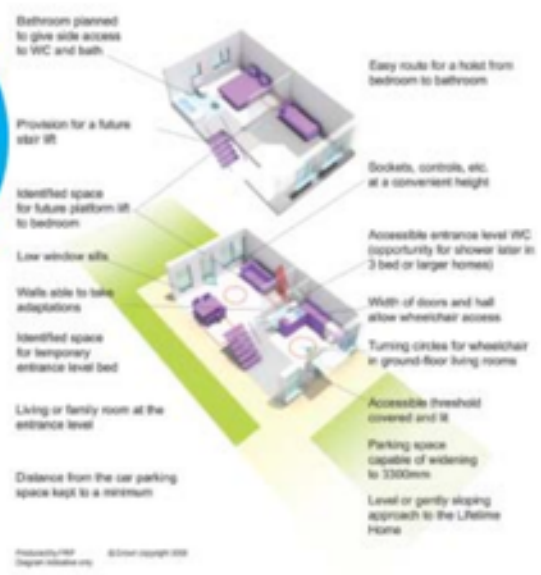
Lifetime Homes Diagram
